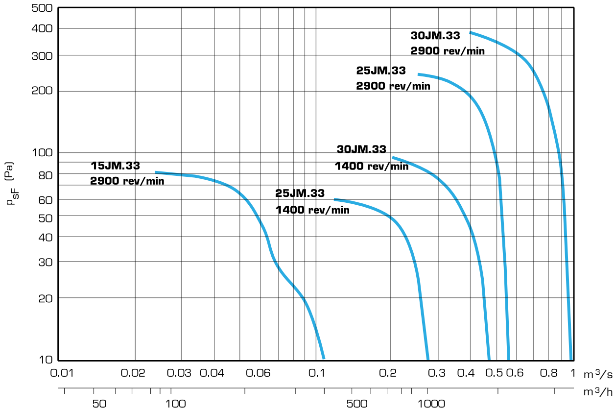
Performance Table - 150-300 mm 380-420v/50Hz/3φ
